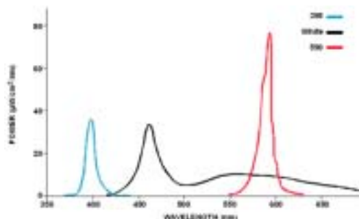
Spectral Output for 395, WHITE, 580nm
