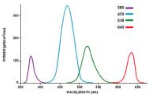
Spectral Output for 380, 470, 518, 648nm
